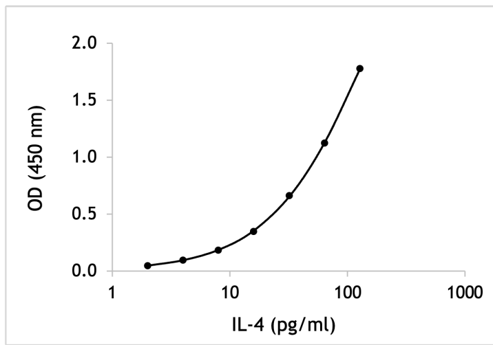
Representative standard curve of rat IL-4
