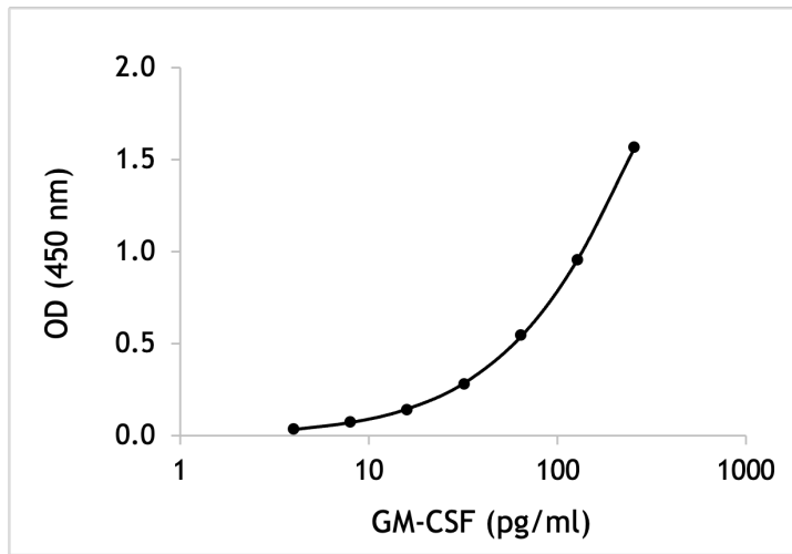
Representative standard curve of monkey GM-CSF
