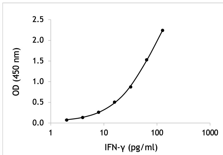
Representative standard curve of monkey IFN- \gamma
