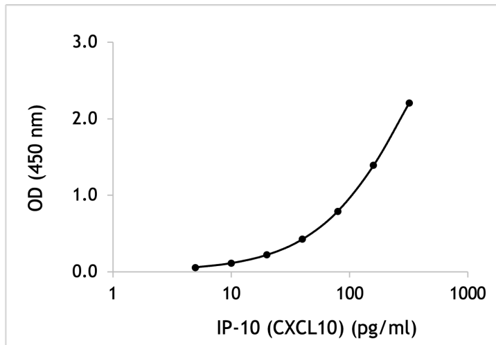
Representative standard curve of monkey IP-10 (CXCL-10)
