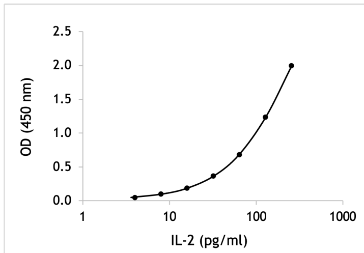
Representative standard curve of mouse IL-2
