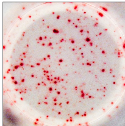
Stimulus: Concanavalin A ( 1 \times 10^5 cells/well)
