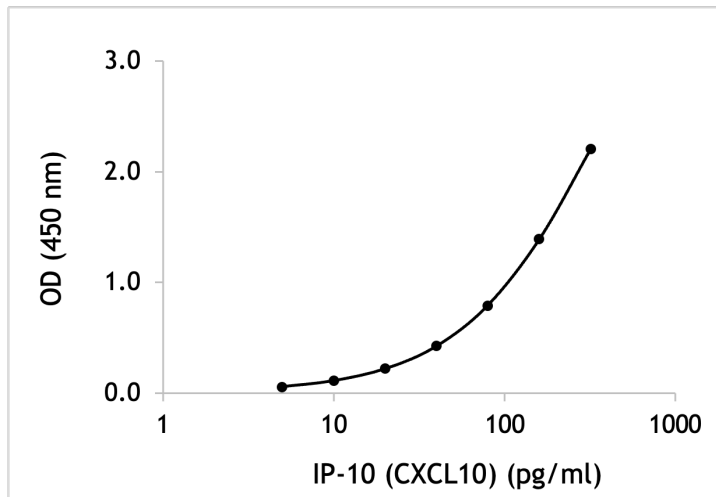
Representative standard curve of human IP-10 (CXCL10)
