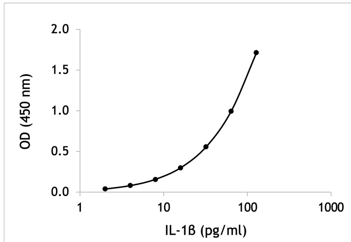
Representative standard curve of human IL-1 \beta
