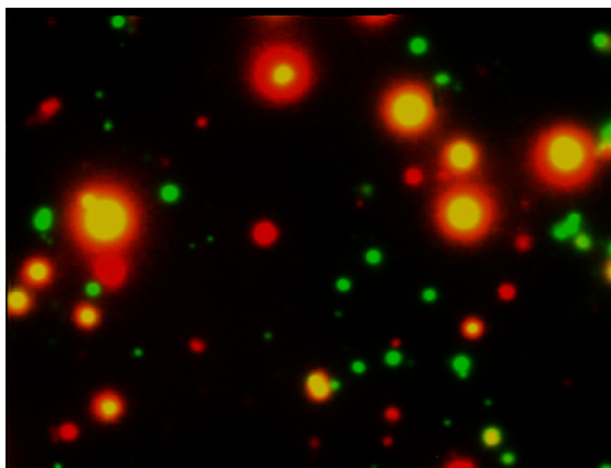
Example of IFN- \gamma /IL-2 specific spots produced by 2.5 \times 10^4 rhesus monkey PBMC In green: IFN- \gamma , in red: IL-2, in yellow: IFN- \gamma /IL-2.
